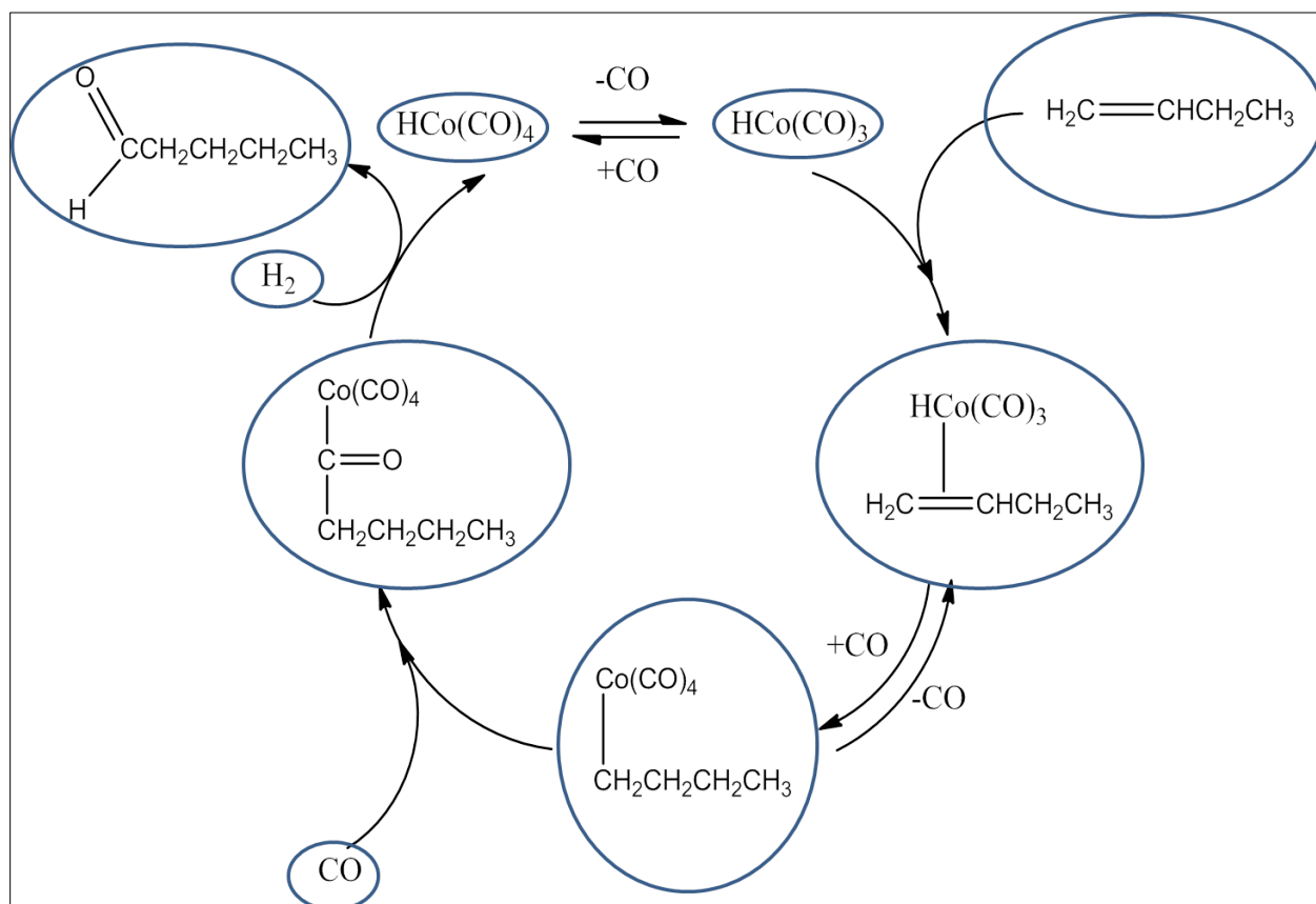
Figure: Catalytic cycle for hydrocarbonylation of 1-butene using cobalt carbonyl catalyst.
