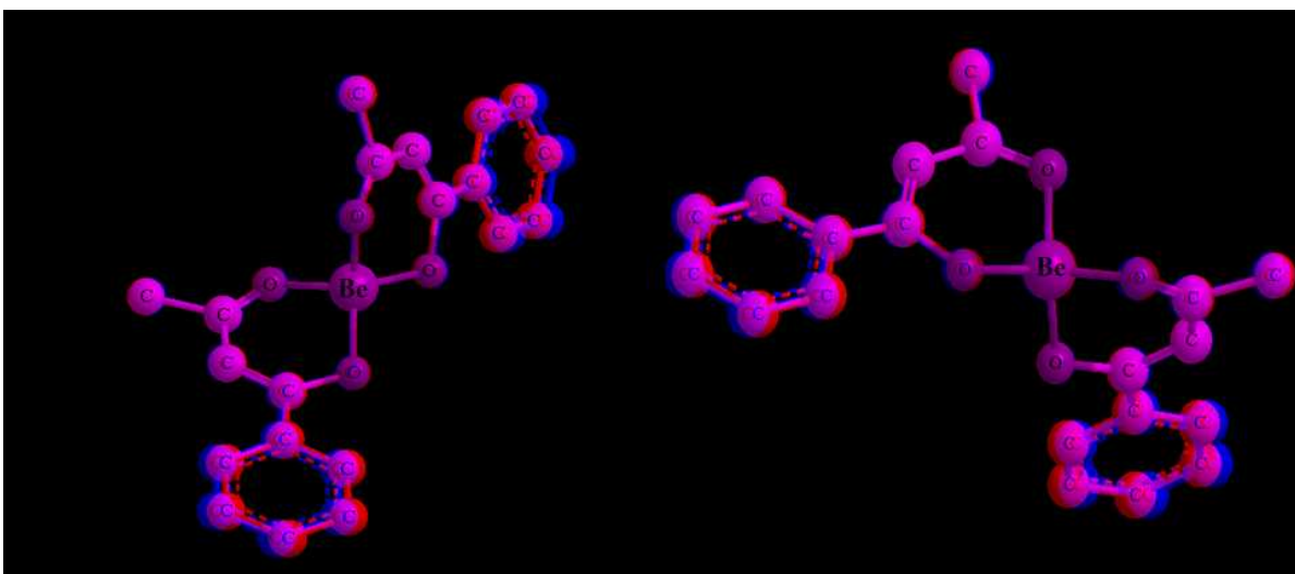
d-bis(benzoylacetonato)beryllium(II)
